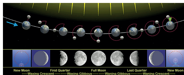
Figure 1. Lunar phases
